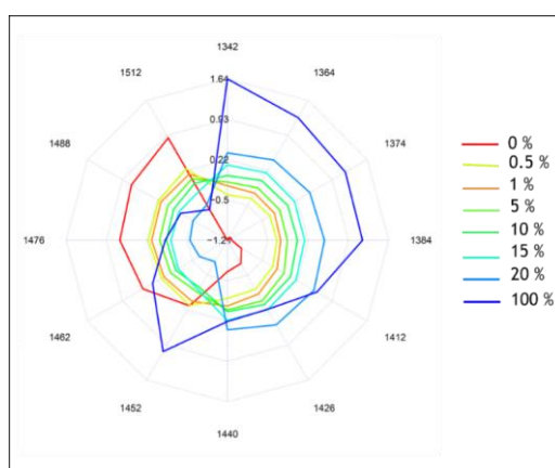
Figure 12: Aquagrams of pure tomato powder extract (0%), pure CF (100%) and Corn Flour (CF) adulterated tomato powder extracts in the concentration range of 0.5–20% and, N=9 each, Spectral range: 1300-1600nm
