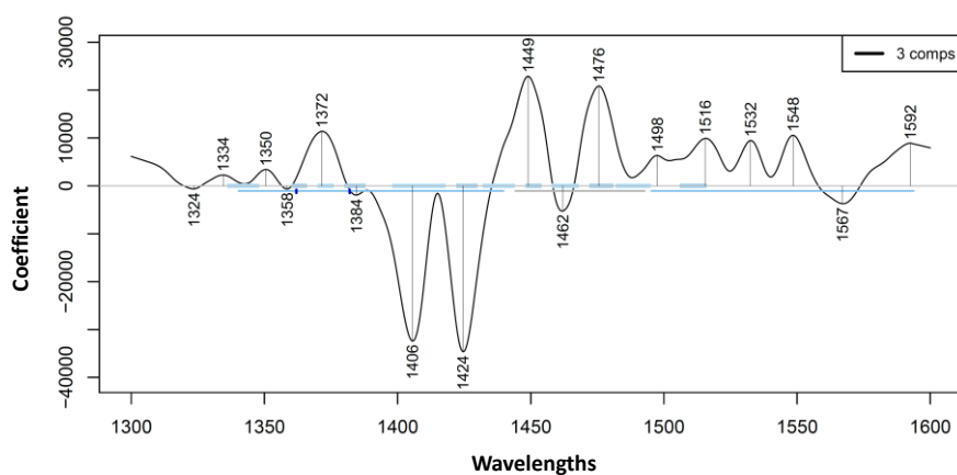
Figure 65: Regression vector of the predictive model of TPC in loyave in the first overtone 1300–1600 nm range.
