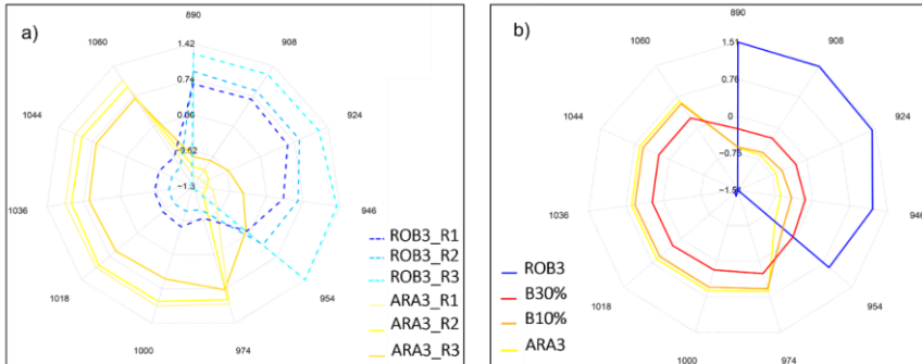
Figure 23: a) Aquagram representation of the spectral pattern of pure Arabica and Robusta extracts at the 2nd overtone (800–1100 nm), N= 9 each; b) Water spectral pattern of marketed blends B10% and B30%, pure Arabica (ARA3) and pure Robusta (ROB3), N= 27 each
