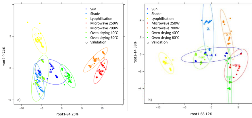
Figure 27: (a) PCA-LDA classification plot of the 1 st set of preserved and ground herbs (rosemary, thyme and marjoram) at the 1 st overtone region (1300–1600 nm) N = 189 , NrPCs =22, (b) PCA-LDA classification plot at the 2 nd overtone region (800–1100 nm), N = 189, NrPCs =16 .
