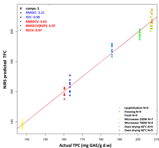
Figure 54: PLSR analysis on sage extracts for the prediction of the TPC (mg GAE/g d.w); N=61, LV=5, Spectral Preprocessing: Savitzky-Golay smoothing (window size 31).
