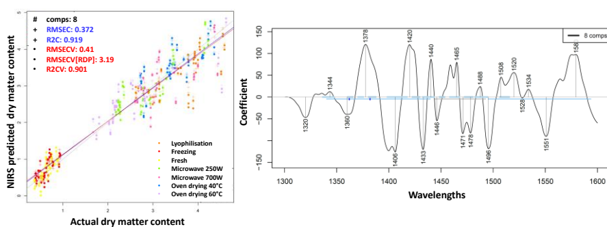
Figure 30: PLSR analysis on the 2 nd set of herbal extracts for the prediction of the dry matter content (mg/ml); Regression vector of the predictive model in the 1300–1600 nm range. N=345, LV=8, Spectral Preprocessing: Savitzky-Golay smoothing (window size 37).
