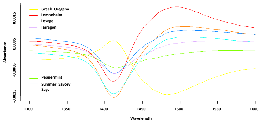
Figure 29: Difference spectra of the fresh herbal extracts obtained by subtraction from the average pure water spectrum in the spectral range 1300–1600 nm.
