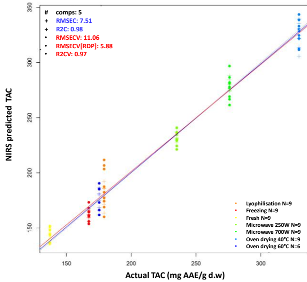
Figure 41: PLSR analysis on Greek oregano extracts for the prediction of TAC (mg AAE/g d.w); N=60, LV=5, Spectral Preprocessing: Savitzky-Golay smoothing (window size 31).
