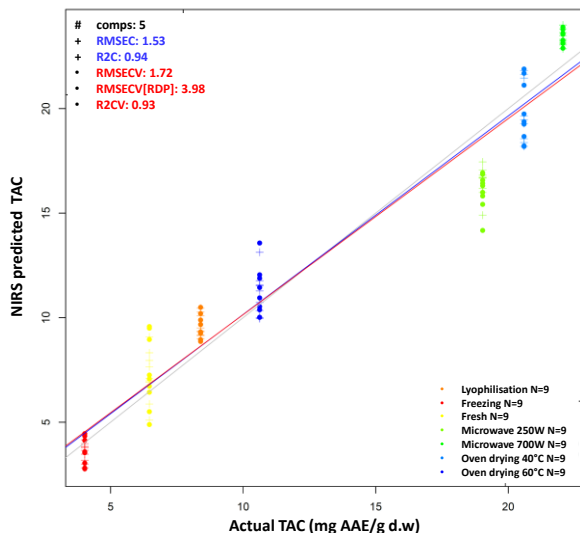
Figure 50: PLSR analysis on peppermint extracts for the prediction of the TAC (mg AAE/g d.w); N=63, LV=5, Spectral Preprocessing: Savitzky-Golay smoothing (window size 31).
