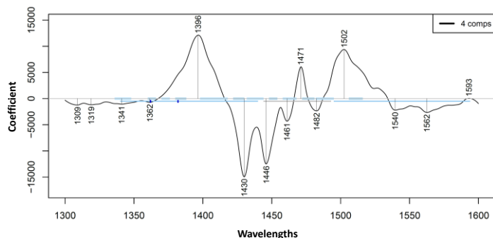
Figure 53: Regression vector of the predictive model of TAC in sage in the first overtone 1300–1600 nm range.
