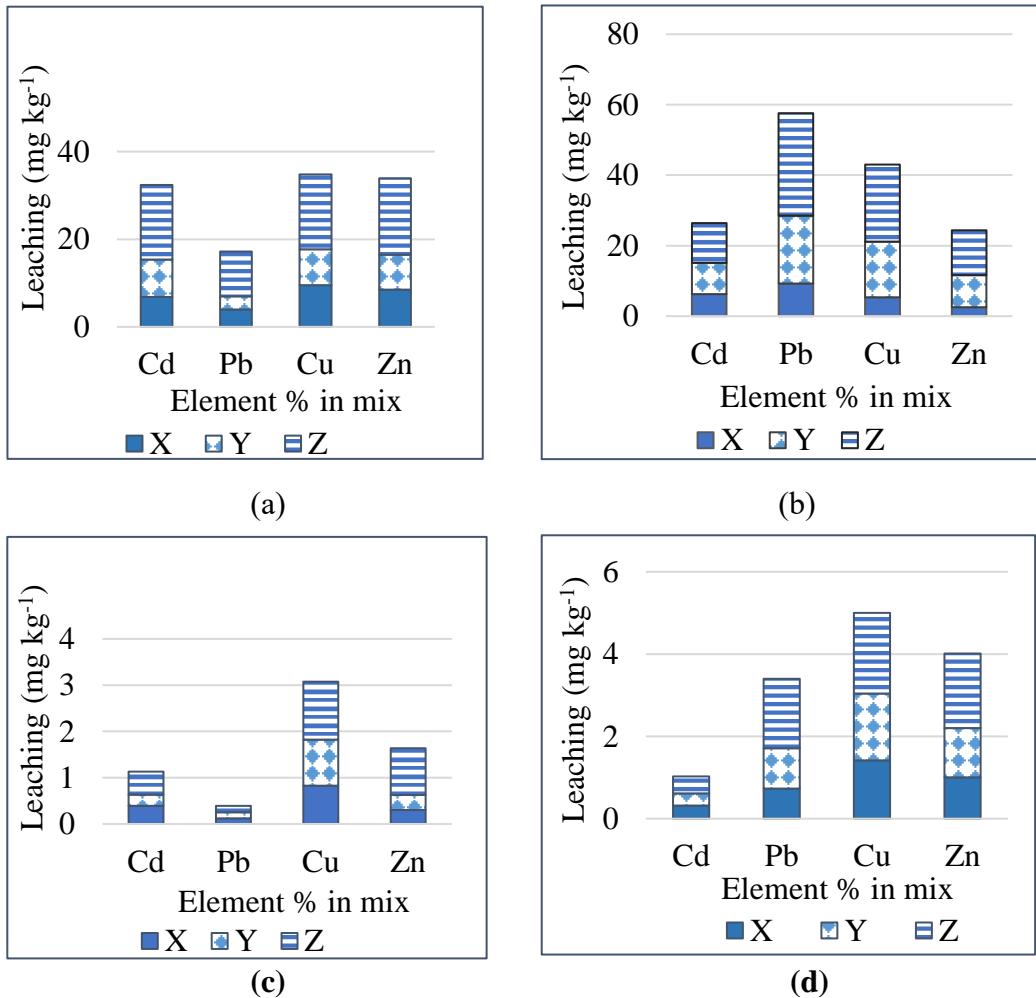
Figure 12. (a) maximum leaching in mulch ash concrete mix (4M HNO 3 ), (b) maximum leaching in paper ash concrete mix (4M HNO 3 ), (c) maximum leaching in mulch 0.43M HNO 3 , (d) maximum leaching in paper 0.43 M HNO 3 . All results are based on average values of 3 replicates of 50 mgL -1 initial concentration of PTEs.
