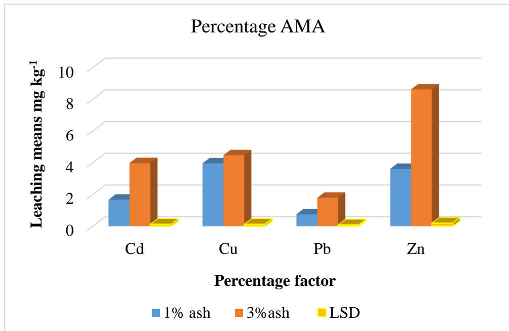
Figure19. AMA ash percentage factor statistical analysis
