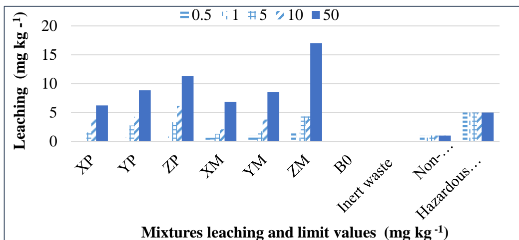
Figure 11. Cd leaching concentrations at 4 M HNO 3 compared to limit values for the individual waste categories.
