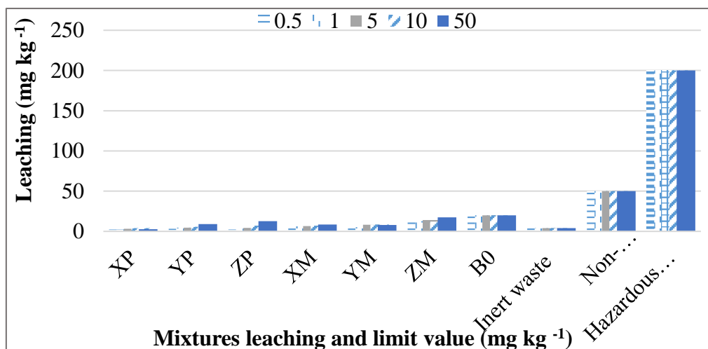
Figure 8. Zn leaching concentrations at 4 M HNO 3 compared to limit values for the individual waste categories.
