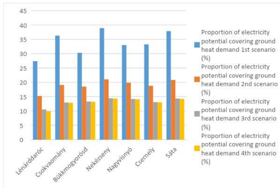
Figure 105. Proportion of electricity potential in different scenarios in Bükk microregion.
