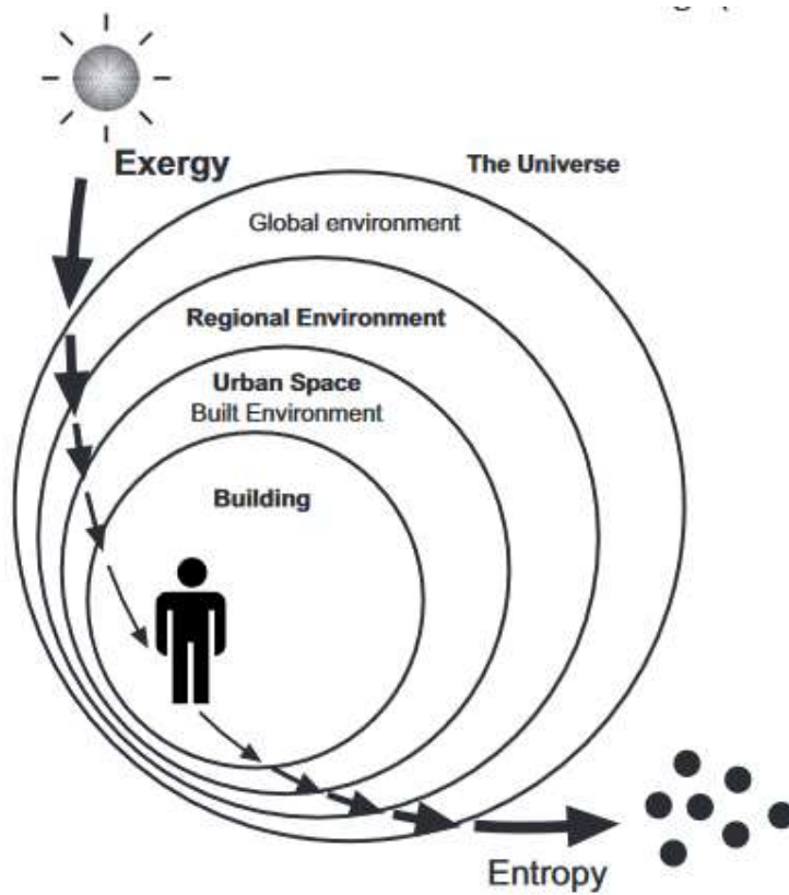
Figure 10. Conceptual illustration of global energy flows. Solar exergy enters the atmosphere and is gradually turned into entropy (Shukuya 2013)
