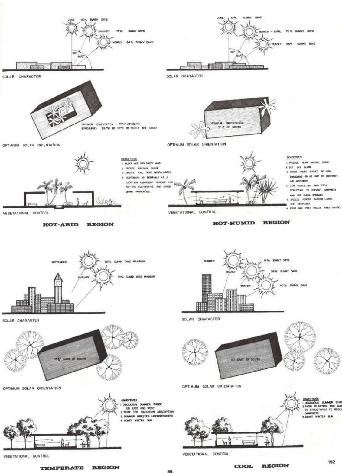
Figure 26. Orientation of buildings in different climate regions taking into account the characteristics of radiation. (Robinette, McClenon 1983)
