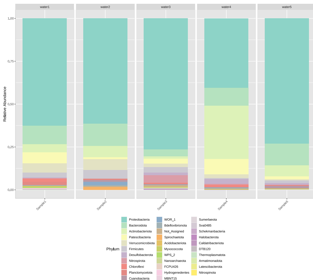
Figure 7 Relative abundance of ASVs regarding each irrigation water sample. ASVs are shown on phylum level
