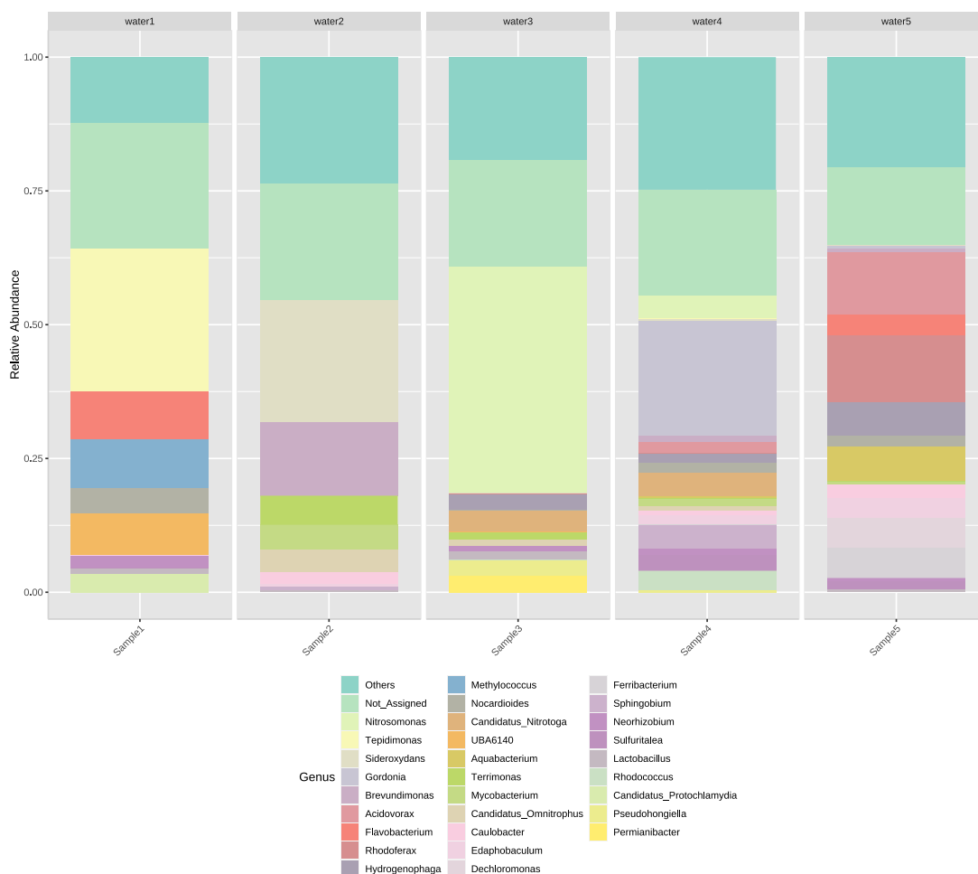
Figure 9 Relative abundance of the 30 most abundantly occurring bacterial genera in the irrigation water samples. The rest of the taxa merged into the group of Others
