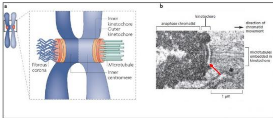
Figure 1. Schematic structure of the central region of the chromosome.
