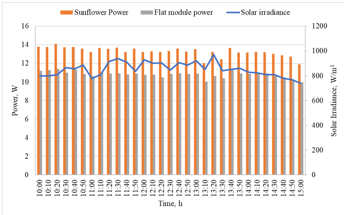
Fig. 4.20. Power generation from the sunflower and the flat PV module ( \alpha=20^\circ )
