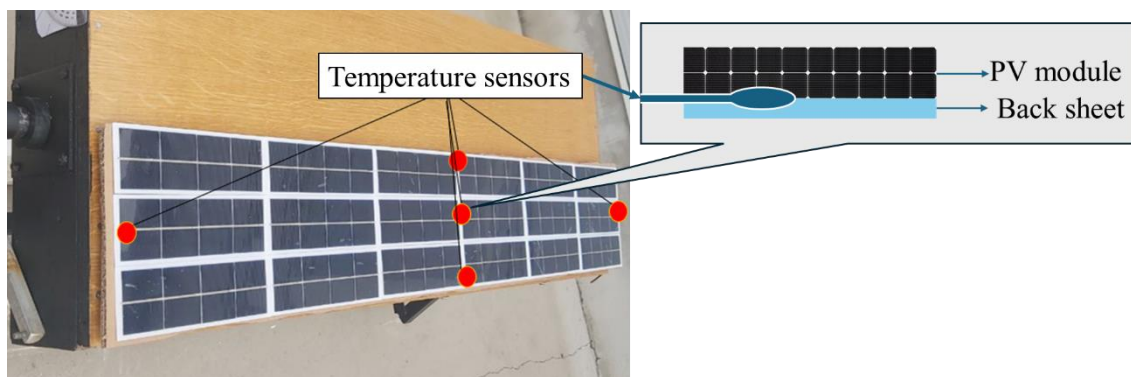
Fig. 3.16. Temperature sensors positions in a flat shape
