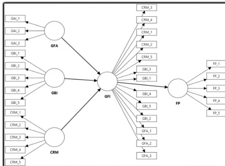
Figure 2: Model Design
