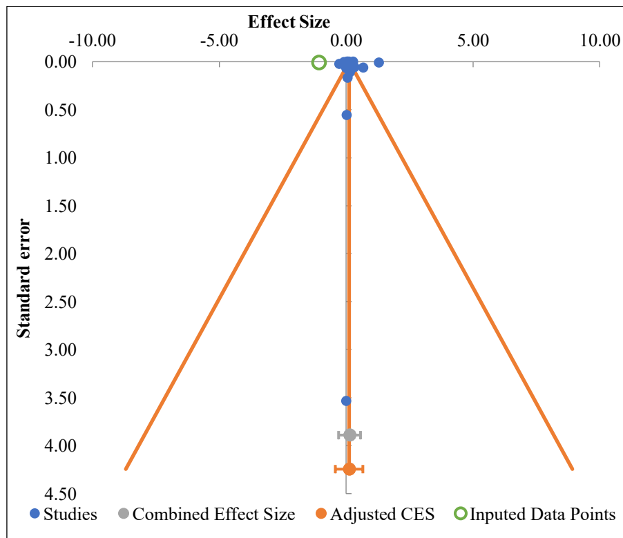
Figure 8: Funnel Plot
