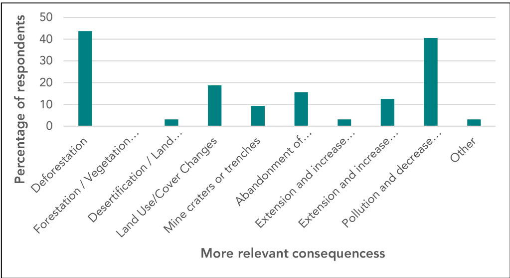
Figure 4.53: Relevant consequences.
