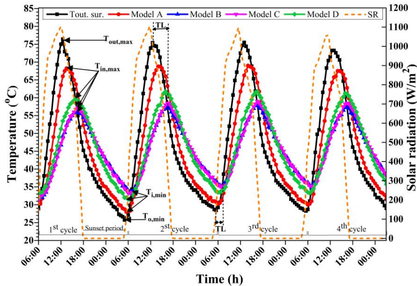
Fig. 4.7. T_{in} vs. T_{out} and SR for tested models (Case II)
