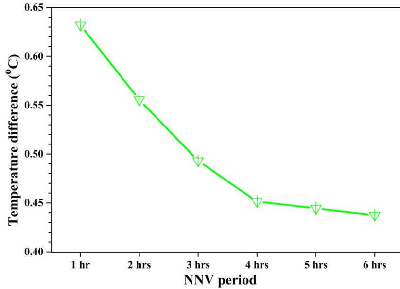
Fig. 4.55. Temperature difference between PCM and reference room during each NNV period
