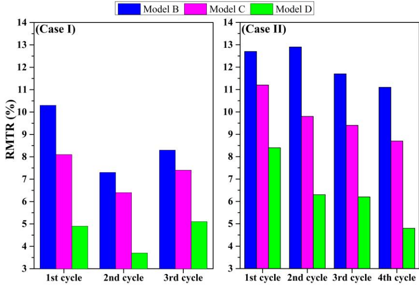
Fig. 4.4. RMTR of PCM models for Case I and Case II
