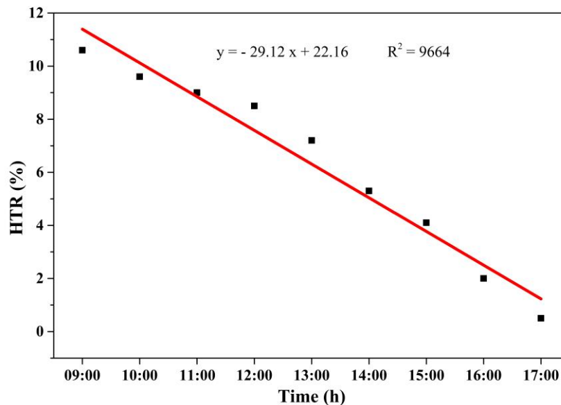
Fig. 4.37. Relationship of the indoor HTR of PCM room with time
