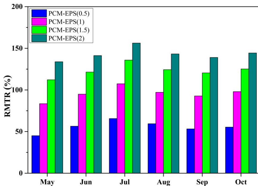
Fig. 4.49. RMTR of PCM-EPS rooms compared with PCM room
