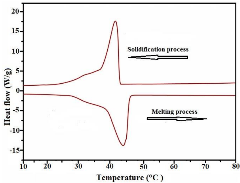
Fig. 3.6. DSC test of used PCM (Ministry of Oil, Midland Refineries Company, 2022)
