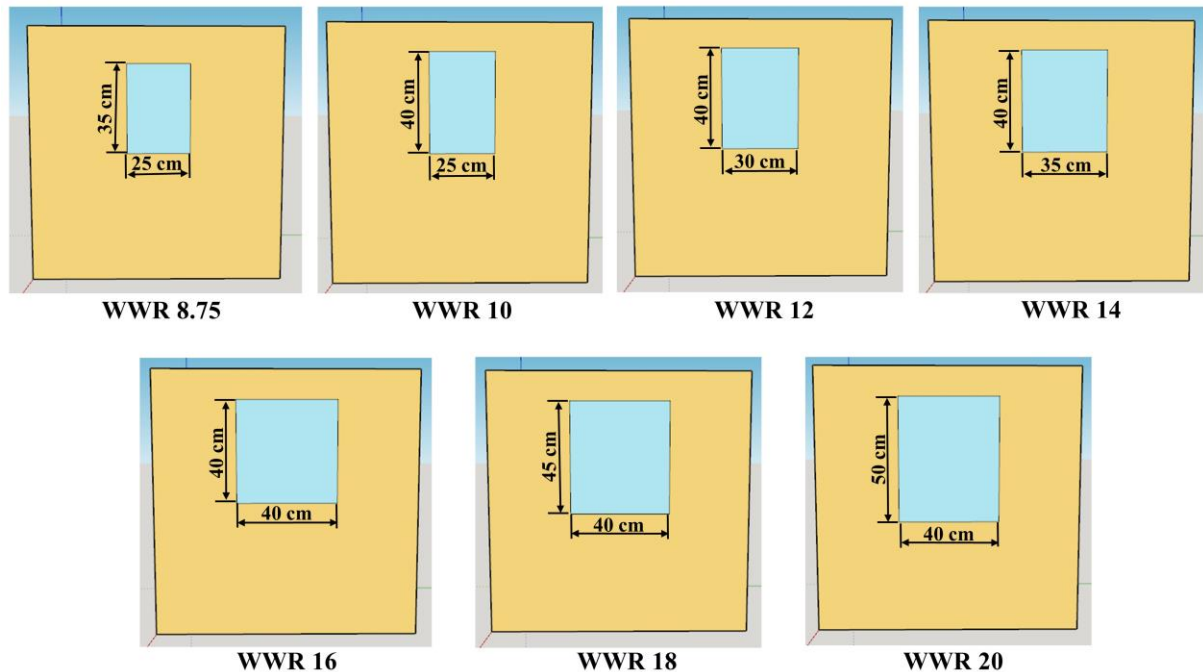
Fig. 3.21. Proposed WWR in the study
