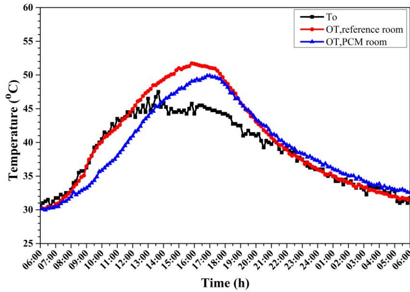
Fig. 4.32. OT variation of reference and PCM rooms
