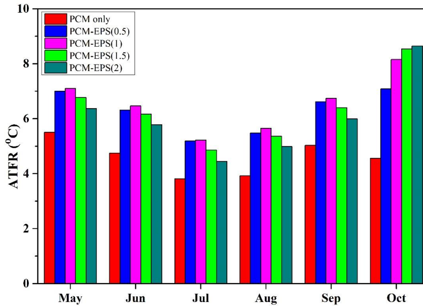
Fig. 4.51. ATFR of modified rooms compared with the reference room
