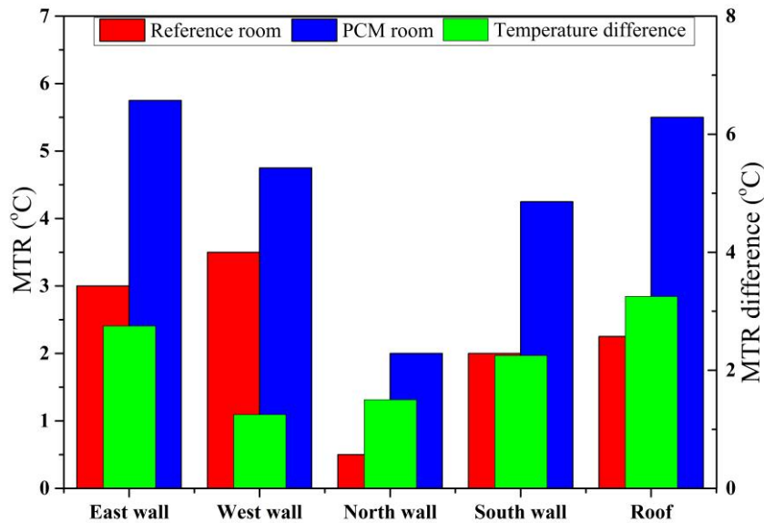
Fig. 4.28. MTR of reference and PCM rooms' elements
