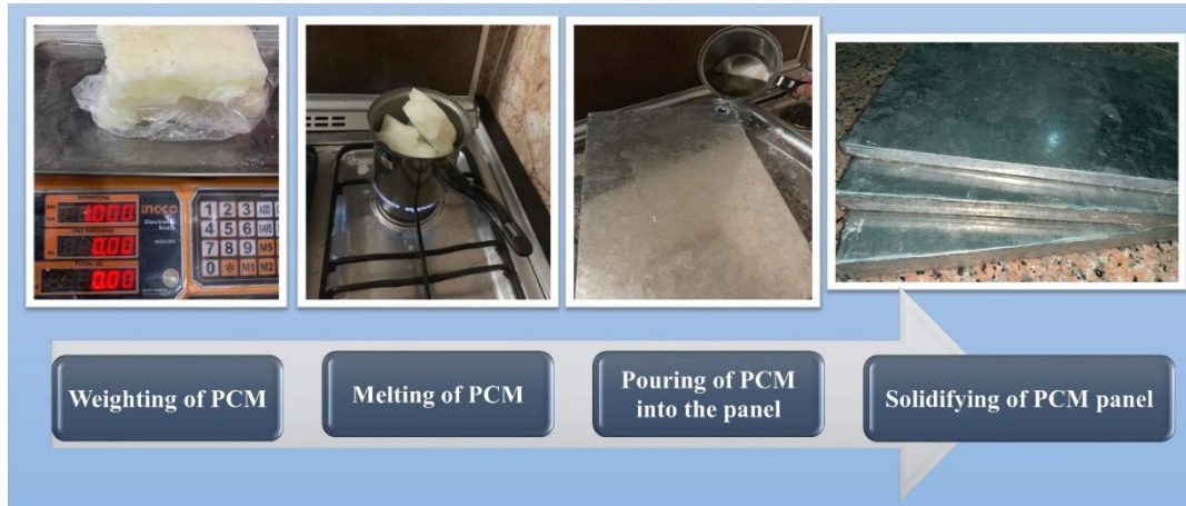
Fig. 3.10. Preparation procedure of PCM panels
