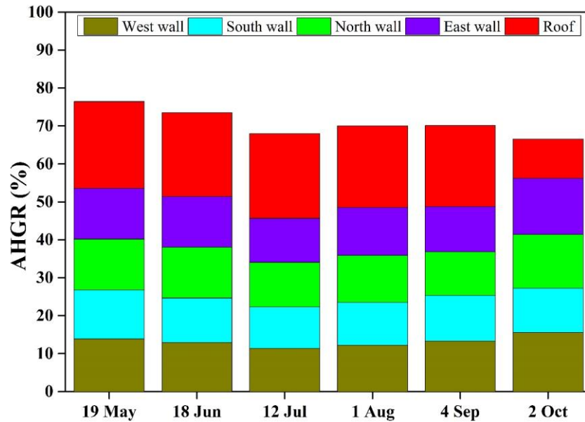
Fig. 4.43. AHGR of envelope elements on the hottest month day
