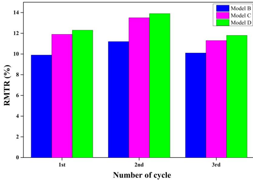
Fig. 4.12. RMTR for tested models
