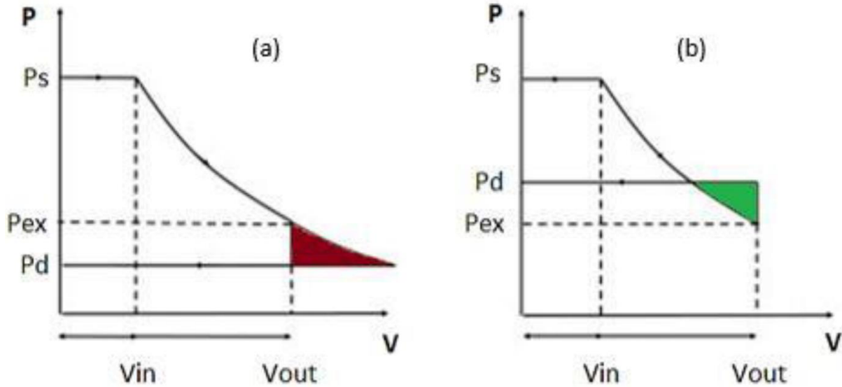
Fig. 2.6. PV graph of scroll expander: a) under expansion, b) over expansion (Campana et al., 2019)
