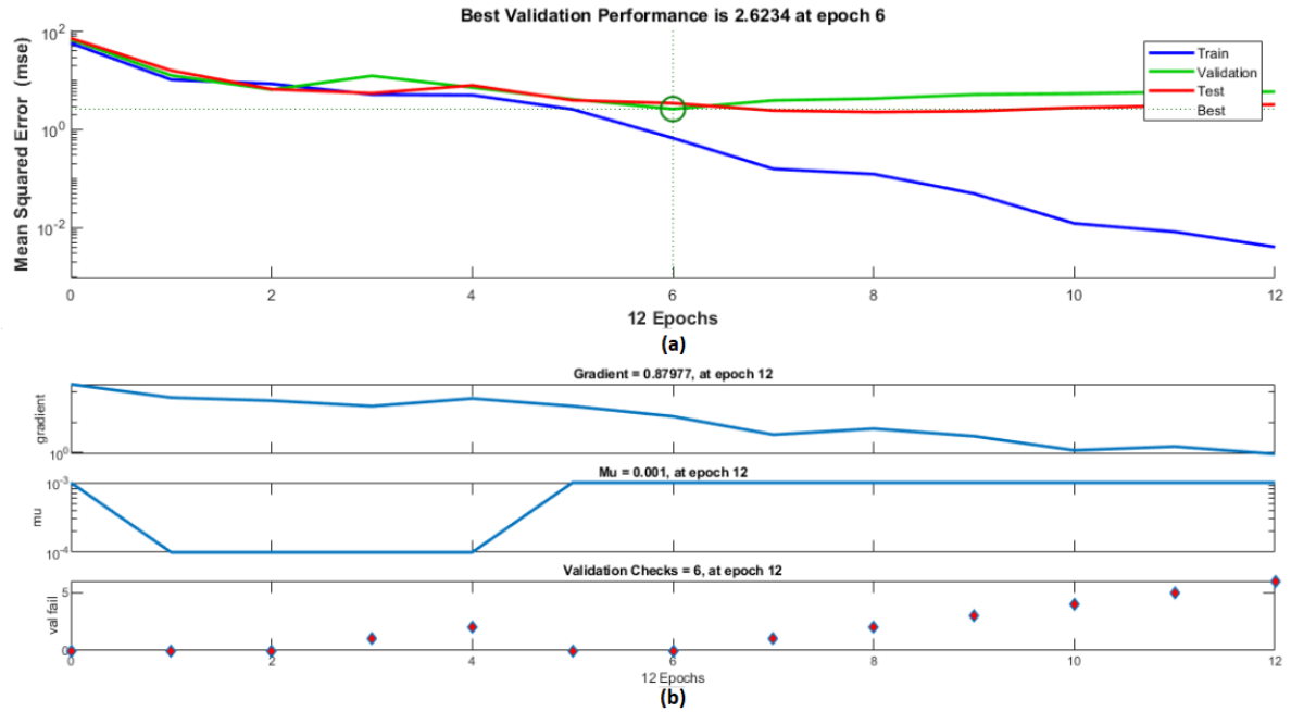
Fig. 4.33 Model performance operation: a) validation, b) epoch
