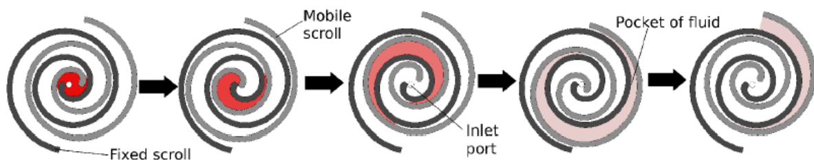
Fig. 2.5. Expansion process in scroll expander (Quoilin et al., 2013)
