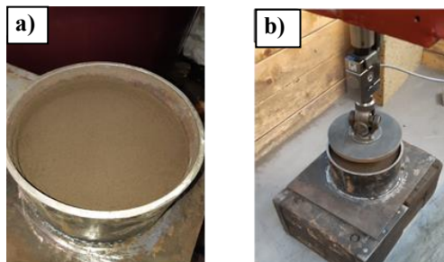
Fig. 2. Small soil bin: a) Filled with soil and b) During the test
