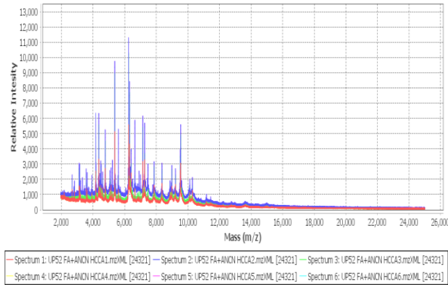
P. lutaonensis MALDI-TOF MS spectra (6 replicates)
