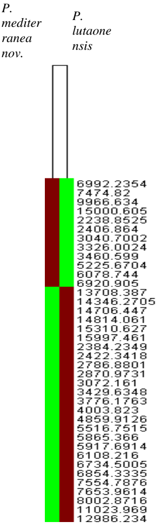
Supplementary figure 7.C Hierarchical clustering analysis of P. lutaonensis and P. mediterranea nov.
