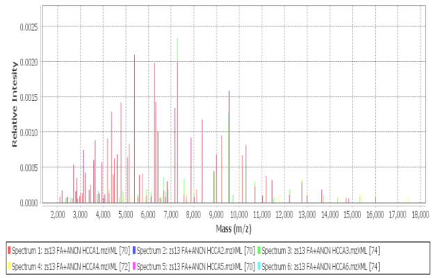
P. mediterranea nov. matched peak list set
