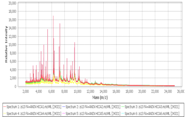
P. mediterranea nov. MALDI-TOF MS spectra (6 replicates)
