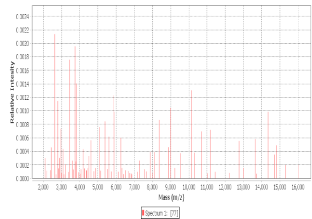
P. mediterranea nov. matched peak list set
