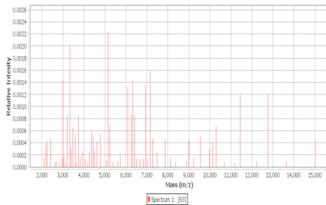
P. lutaonensis matched peak list set
