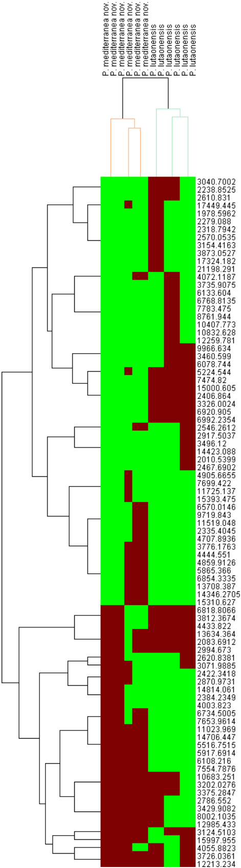
Supplementary figure 7. A Dendrogram generated from hierarchical cluster analysis of MALDI-TOF mass spectra of P. lutaonensis and P. mediterranea nov. (6 replicates)
