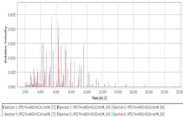
P. lutaonensis labeled peak list (6 replicates)
